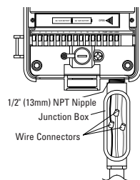
FIGURE 23: AC Wiring Using Junction Box
