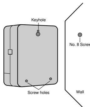
FIGURE 19: Mounting the Controller
